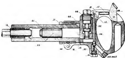
Fig. 4990. Green Chipping and Cantking Hammer, Class B, with Outside Trigger. Dayton Pneumatic Tool Co.
